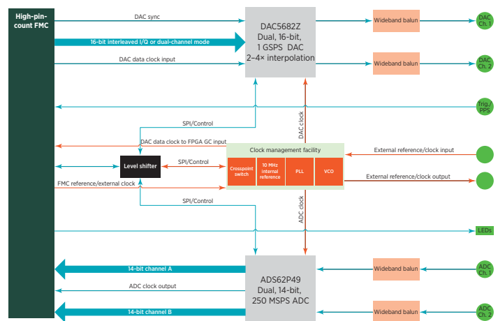
ADAC250 functional block diagram
